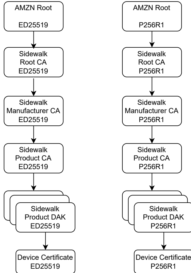
Fig. 4.2 Certification path
