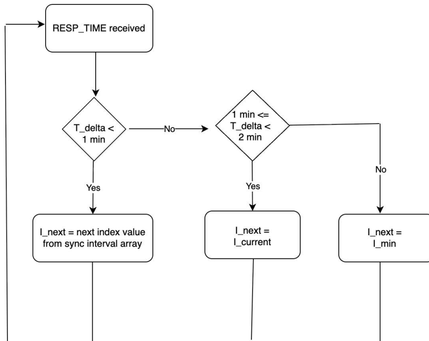
Fig. 8.3 Time sync maintenance Interval
