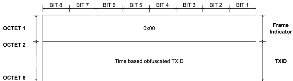
Fig. 6.10 BLE Beacon - Application Specific Data - Time based connection request and presence detection
