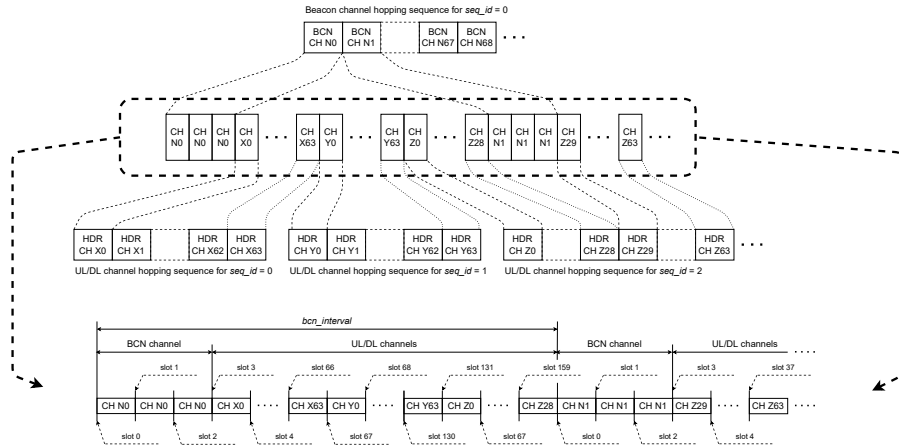
Fig. 5.54 SubG-FSK connection - Channel hopping usage
